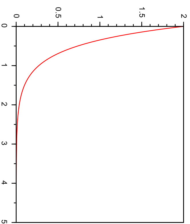
lambda=2
